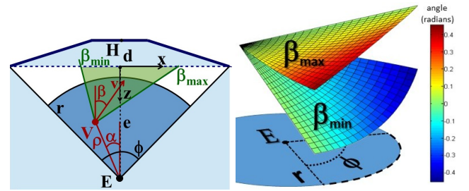
Figure 5: Constrained exploration. Left: the workspace for exploration is defined by the starting view point, the horizon position and the field of view. The view matrix can be parametrized with three values: a distance \rho , and two angles \alpha, \beta , for representing the view point V and the view direction \hat{v} . Right: the 3D representation of the constraints for the viewing direction angle \beta .
