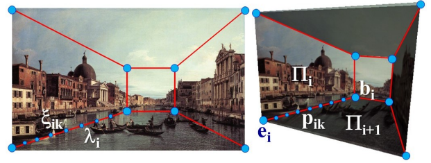
Figure 4: Semiautomatic correction. The scene model can be tuned by modifying the 2D positions of 8 control points. The system automatically computes the optimal scene parameters matching the scene plane intersections to the selected line segments.
