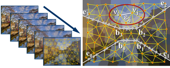
Figure 3: Automatic scene fitting. Left: a multiresolution superpixel representation is obtained by repeated application of the SLIC clustering algorithm, and a hierarchy of graphs is built on it. Right: the scene representation is fitted by employing a graph-cut strategy for minimizing a penalty function computed along the edges of the graph.
