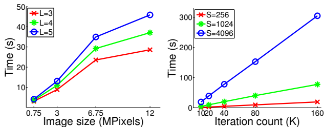
Figure 9: PEEP construction. Left: graph construction times as function of image size (with varying number of levels L ). Right: global optimization times as function of number of iterations (with varying number of superpixels S = 2^{16-2(L-1)} )
