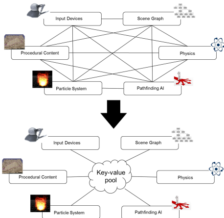
Figure 1: Figure 1: Conversion from many-to-many dataflow to many-to-one dataflow [LWZ14]
