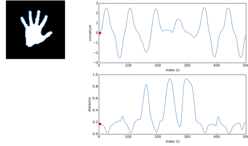
Figure 8: Curvature and distance features for a sample gesture. The feature values have been plotted starting from the red point and proceeding in clockwise order along the hand contour.
