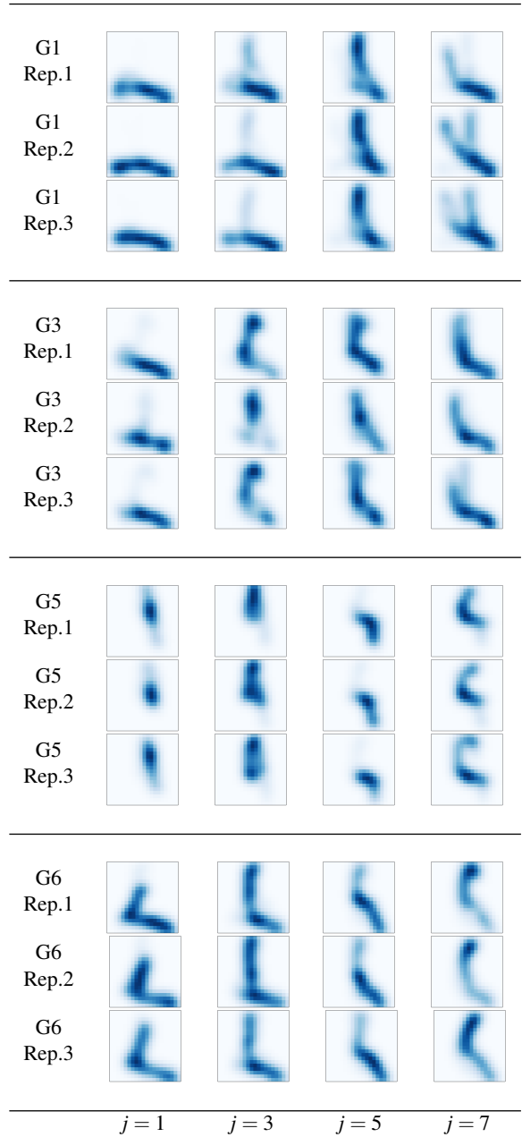
Figure 11: The figures shows 4 different slices of the feature array \mathbf{A} for 3 different repetitions of 4 different gestures (i.e., gestures G1, G3, G5 and G6). Notice how the slices are similar for different repetitions of the same gesture and very different among different gestures.
