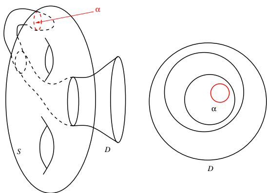
Figure 3: Decreasing the number of components of D \cap \mathcal{S}
