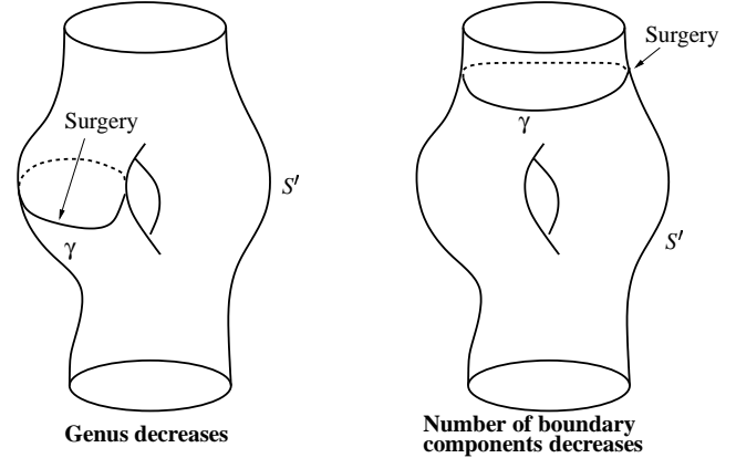
Figure 6: The effects of a surgery on \mathcal{S}'
