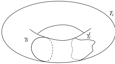
Figure 5: Torus on the boundary of \tilde{M}
