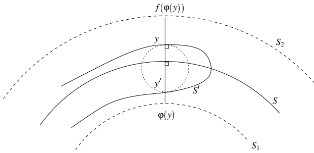
Figure 1: Proof of corollary 3.3.
