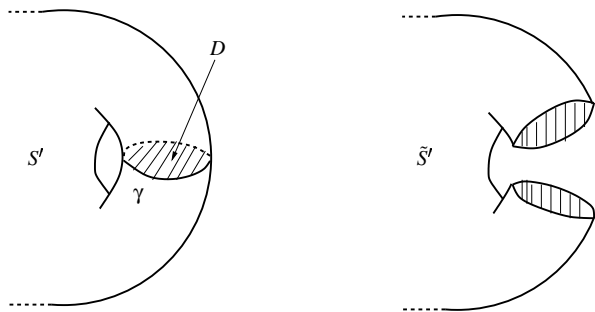
Figure 2: Surgery along a compressing disk
