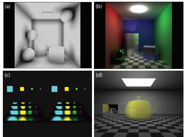
Figure 4: Output of the graduate lab session tasks. a) Ambient occlusion. b) Unidirectional path tracer using importance sampling. c) Comparison of BRDF versus light importance sampling. d) Volumetric rendering.
