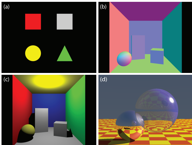
Figure 3: Output of the first (a-c) and second (d) undergraduate lab sessions. a) Unlit shading of supported primitives. b) Cornell Box using normal vector colouring and c) Lambertian shading. d) Whitted-style ray tracer [Whi80].
