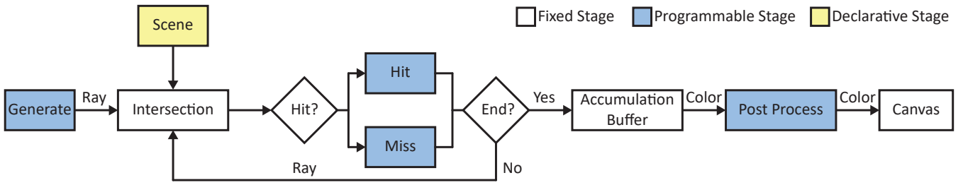
Figure 2: High level overview of the Rayground pipeline. Shaded polygons correspond to programmable stages. Rays are submitted as waves and intersection results are provided to the next stages through appropriate API calls.
