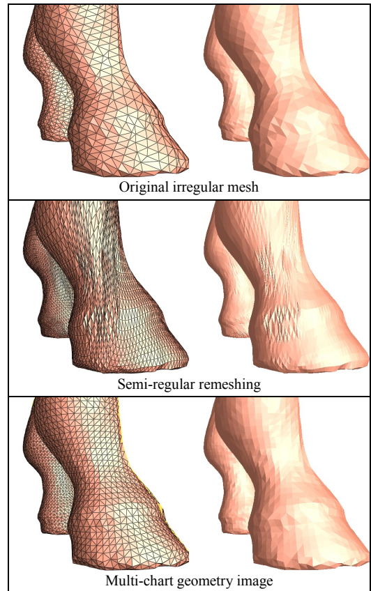
Figure 12: Horse close-up showing improved sampling uniformity of MCGIM over semi-regular remeshing.
