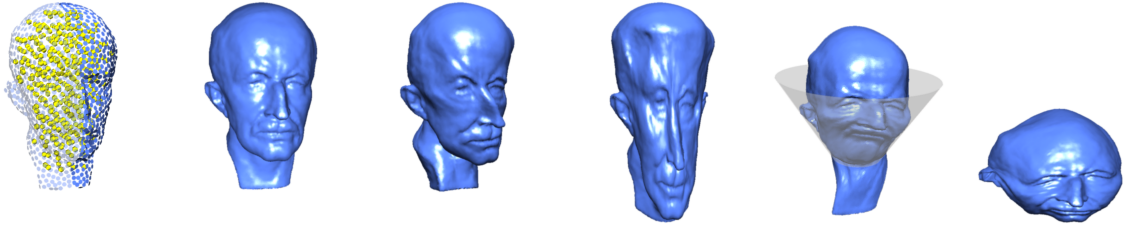
Figure 1: Left two images: to compute realistic deformations, we represent both the physical volume elements ( phyxels ) and the surface elements ( surfels ) as point samples. Right four images: With our system we can model and animate elastic, plastic, melting and solidifying objects.
