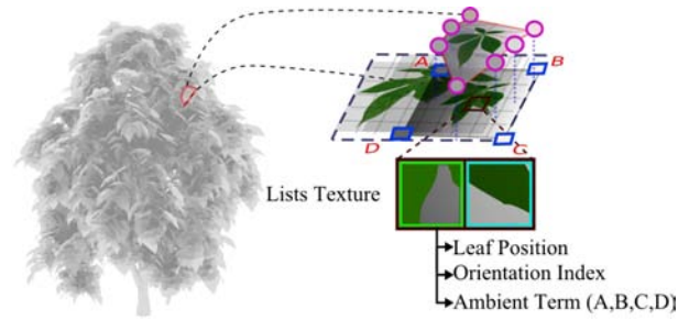
Figure 11: Ambient term generation for the multi-layer leaves representation is encoded as a new field of the List Texture at the leaf level. The small squares represent the actual ambient occlusion values at the corresponding vertices.
