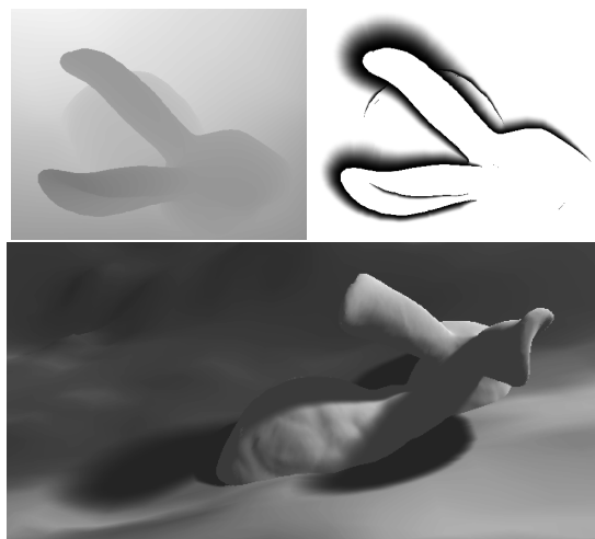
Figure 3: An example shadow map (top left), corresponding penumbra map (top right), and the final rendered result. (Also see color plate.)
