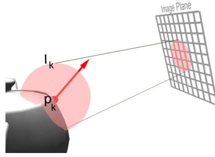
Figure 2: The sphere I_k around the position \mathbf{p}_k of the record k is splatted on the image plane. For each point within the sphere splat, the contribution of record k is accumulated into the radiance splat buffer.
