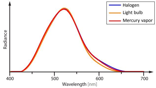
Figure 5: Re-radiation spectrum for phosphorescent stickers after excitation by different types of light sources. The curves have been linearly scaled by their respective average value.
