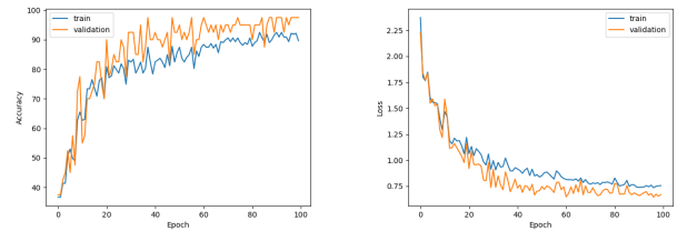
Figure 10: GCN training accuracy and loss obtained on the Configurators CAD dataset.
