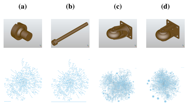
Figure 6: Examples of CAD models in the dataset and their respective generated graphs. 3D models belonging to the same class, (a)-(b) and (c)-(d), can be represented by graphs with similar structure even if they are visually different such as (a)-(b) or by graphs with different structure even if they are visually similar such as (c)-(d).
