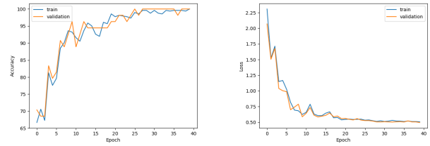
Figure 9: GCN training accuracy and loss obtained on the Traceparts CAD dataset.
