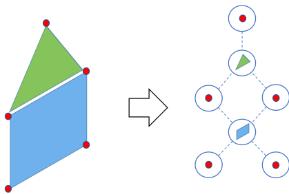
Figure 2: Example of conversion from the geometric information of a STEP file to a graph structure.
