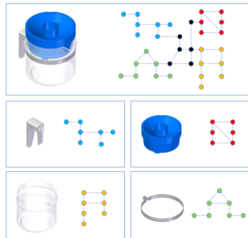
Figure 3: Example of the decomposition into components of a CAD file and its related sub-graphs.
