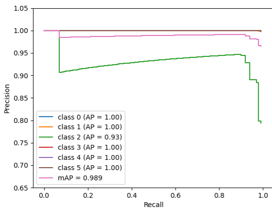
Figure 11: Precision-recall curve for the retrieval of CAD models with features vectors extracted from the softmax layer and cosine distance as metric for comparing feature vectors of the first dataset.
