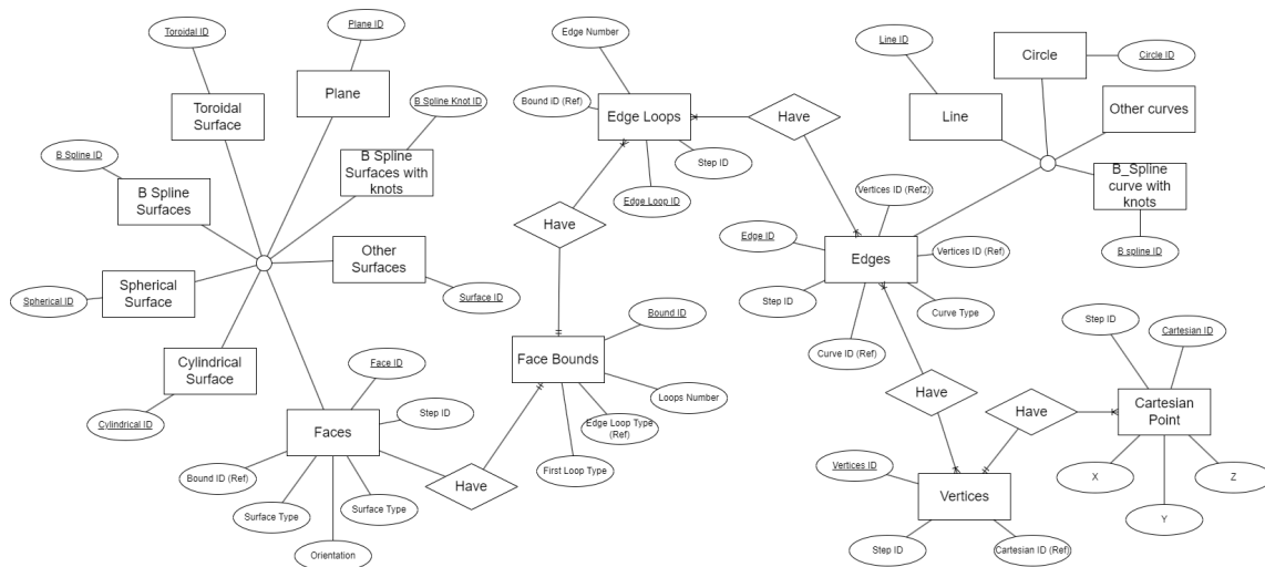
Figure 1: Entity relationship diagram that shows some of the entities defined in the STEP standard.
