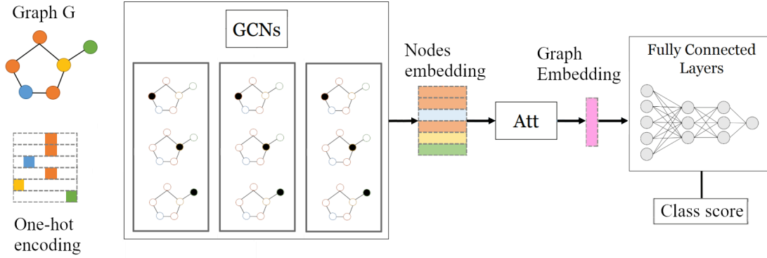
Figure 4: Structure of the proposed GCN network. The GCN layers generate the nodes embedding that are then passed together through an attention mechanism, which generates an embedding of the entire graph. Two fully connected (FC) layers and the softmax function lead to the classification score.
