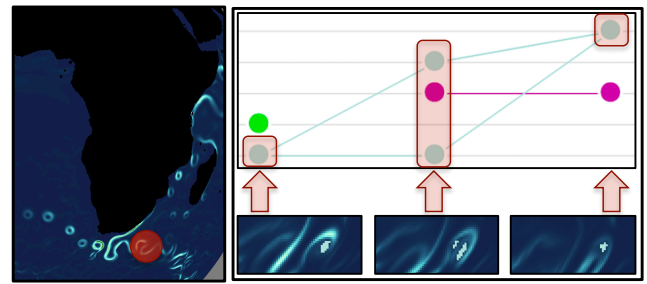
Figure 6: Closeup view of Eddy Tracking Graph from Figure 1(c) shows the light blue eddy splitting into two, and merging back into one. Eddy merges are more rare than eddy splits in the South Atlantic Ocean, due to the turbulent nature of the currents in the region. In this example, a small eddy splits into two, then merges back into one in the region of the Agulhas Return Current.
