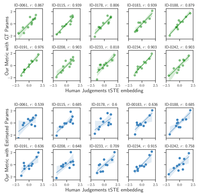
Figure 9: Correlation between the ordering provided by the Human Judgments ( x -axis) and our drape similarity metric with (top) the Ground Truth simulation parameters ( y -axis), and (bottom) the estimations of our model. We plot z-scores instead of the raw distances to help visualization.
