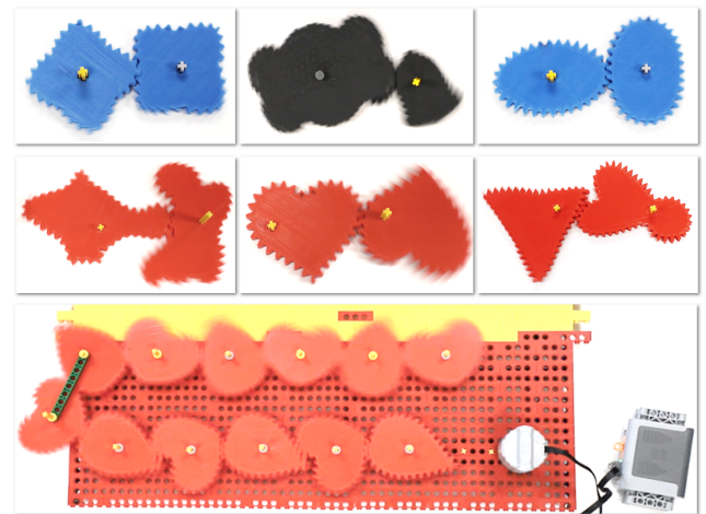
Figure 18: Our 3D-printed non-circular gears. Top: SQUARE-SQUARE, BELL-CANDY & ELLIPSE-ELLIPSE; middle: FISH-BUTTERFLY, HEART-HEART & TRIANGLE_BELL-SUNNY_DOLL; and bottom: a gear train composed of six pairs of DROP-HEART.
