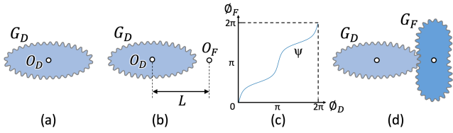
Figure 6: Our approach to compute the mating gear. Given (a) G_D and K = 1 , we first locate (b) G_F 's rotation center O_F , then compute (c) the transmission function and (d) G_F 's geometry.
