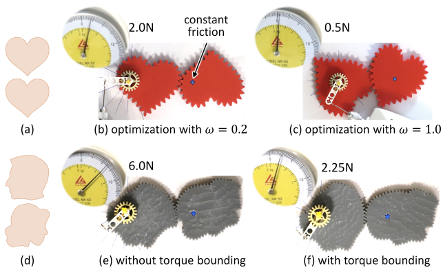
Figure 19: Experiments on maximum instantaneous torque required to drive the gears. From the same input shapes (a&d), HEART-HEART gears generated with (b) \omega = 0.2 and (c) \omega = 1.0 ; and BOY-GIRL results generated (e) without and (f) with torque bounding. The torque is measured by a force gauge with a fixed arm of force (see the numbers in the yellow dial plate).
