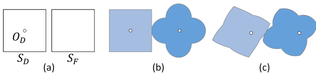
Figure 10: (a) Input shapes with rotation center O_D marked on S_D . Mating gears generated using our (b) first and (c) second attempts.
