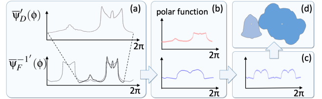
Figure 13: Constructing mating gears for K = 2 . We match (a) \bar{\Psi}'_D(\phi) with 1/K of \bar{\Psi}'^{-1}'_F(\phi) , (b&c) duplicate the resulting polar function (in blue) of the follower gear K times, normalize it, and then (d) compute the boundary curves of the gears.
