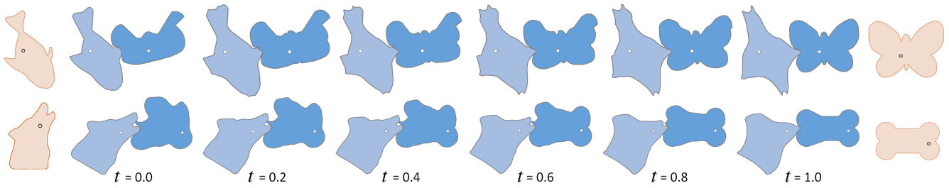
Figure 17: Preference on preserving one particular input shape can be expressed by adjusting the value of t in Equation 14. Note that the rotation centers of the gears are fixed in these optimizations (see the dots in the input shapes). Top: FISH-BUTTERFLY; bottom: DOG-BONE.
