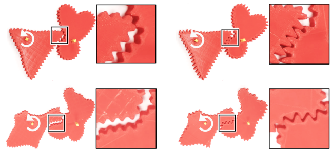
Figure 20: Gears generated with regular and customized teeth. Left: gears with regular teeth could lose contact during motion transfer (see the zooming views). Right: gears with customized teeth could maintain unceasing contact.
