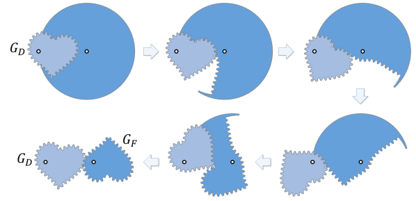
Figure 7: The rotate-and-carve approach to generate G_F from G_D .
