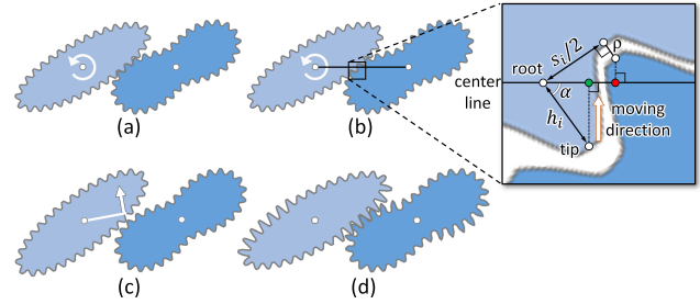
Figure 14: Constructing teeth on gears (a) without and (b) with tolerance, showing that the tolerance is small. (c) Gears with regular teeth could lose contact during motion transfer. (d) We create customized teeth with non-uniform shape for better gear meshing.
