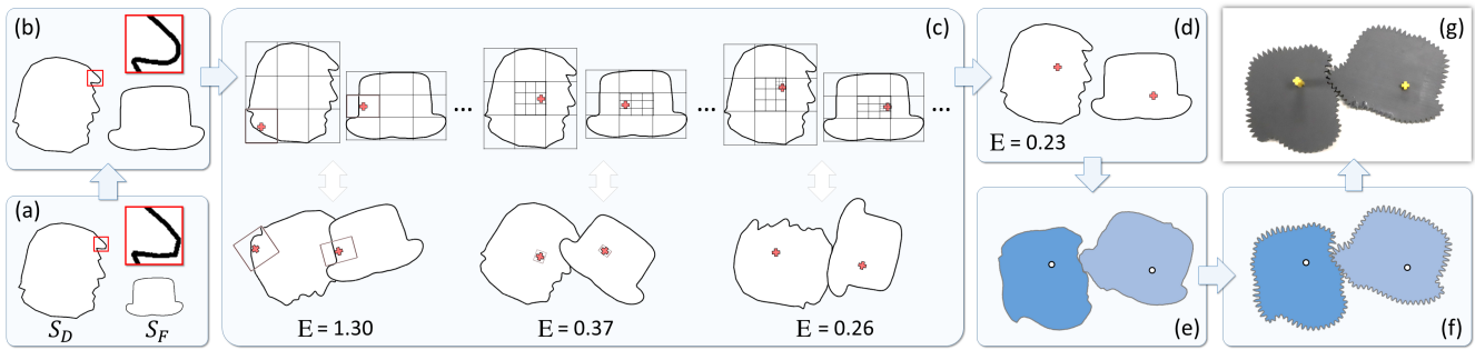
Figure 9: Overview of our approach: (a&b) smooth and normalize the input shapes; (c) recursively sample and evaluate rotation center candidates; (d) choose the ones with minimal E ; (e) construct the gear shapes; (f) generate teeth; and (g) fabricate the resulting gears.
