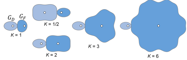
Figure 5: Example non-circular gear pairs with different transmission ratio K . Teeth are omitted for better boundary visualization.
