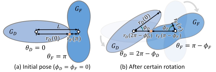
Figure 4: A mating gear pair without teeth for better visualization. The contact point (orange dot) is always on the line between the two rotation centers.
