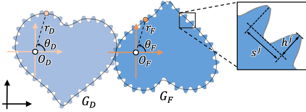
Figure 3: Geometric parameters of a non-circular gear pair. As a convention, we color the driver ( G_D ) and follower ( G_F ) in light blue and dark blue, respectively, throughout the paper. The local coordinate system of G_D ( G_F ) is colored in light (dark) orange, and the world coordinate system is colored in black.
