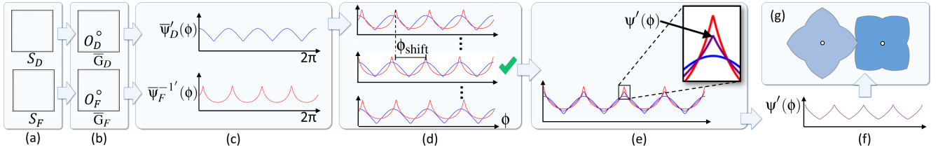
Figure 11: Our approach to compute mating gears from (a) input shapes. We first (b) locate a rotation center in each input shape, (c) compute the derivatives of their transmission functions, (d) find the shift angle to align the two derivatives, (e&f) obtain the derivative of the target transmission function by interpolating the two aligned derivatives, and lastly, (g) generate boundary curves (shapes) of the resulting gears.
