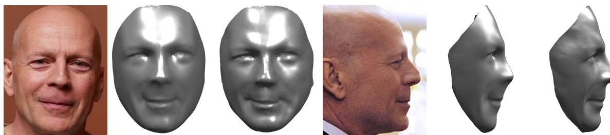
Figure 1: We introduce silhouette constraints to improve the quality of unconstrained 3D face reconstruction. Here, we show a comparison between the state of the art approach by Roth et al. [RTL15] and our technique. The 2nd and 5th column are the results from [RTL15], the 3rd and 6th column are our results. Note how our approach follows more faithfully the silhouettes of the input images, especially around the nose region.
