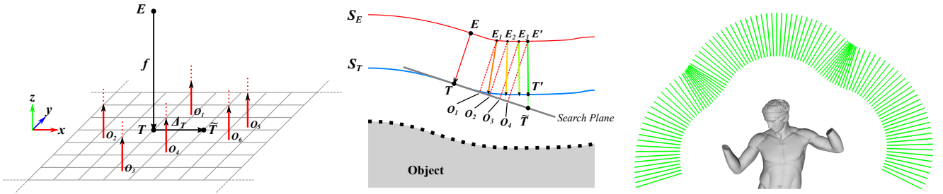
Figure 7: Left: the space of points O_i used to perform ray casting operations. Center: simplified 2D section for the searching algorithm. Right: series of camera eye-target vectors generated with fixed step panning operations along one direction.
