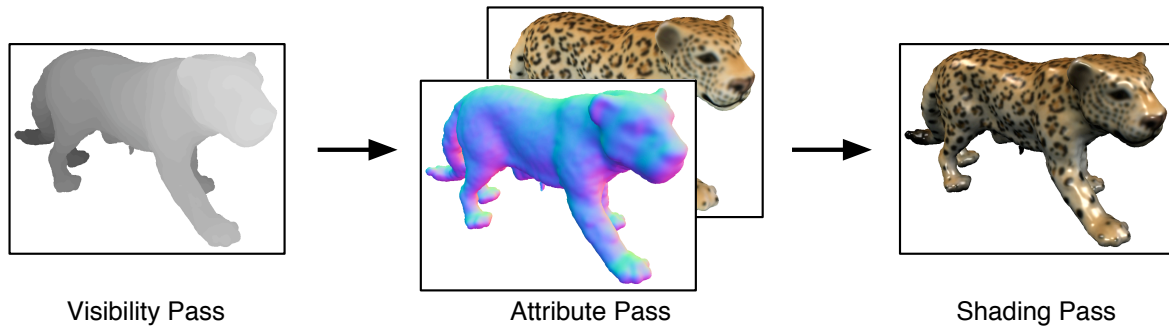
Figure 1: The deferred shading pipeline for GPU-based splatting. The visibility pass fills the z -buffer, such that the attribute pass can correctly accumulate surface attributes, like color values and normal vectors, in separate render targets. The final shading pass computes the actual color value for each image pixel based on the information stored in these render targets.
