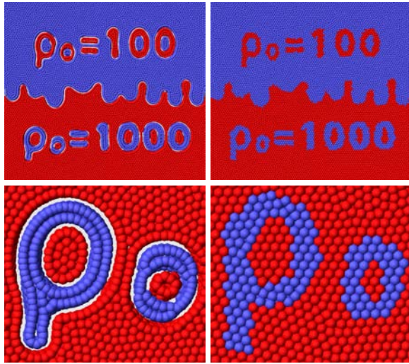
Figure 2: In contrast to the new method (right), the use of standard SPH produces a spurious interface tension and a gap between two fluids with a density contrast (left).
