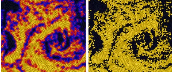
Figure 4: Standard SPH density (left) versus our corrected density (right). The two fluids have rest densities of 1000\text{kg/m}^3 and 100\text{kg/m}^3 . The computed density is color-coded with yellow being 1000, red 700, blue 400, and black 100, respectively.
