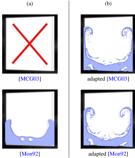
Figure 5: Two fluids with a density ratio of 10 are simulated with two different pressure force equations, (a) on the left using the original formulations, and (b) on the right using our adapted equations. While the standard formulations result in instability (upper left: Equation 5) and spurious tension problems (lower left: Equation 7), these problems can be overcome by using our modified equations (Equation 14 and Equation 19).
