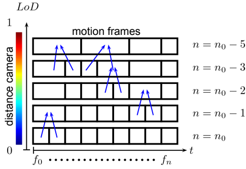
Figure 14: Motion LoD.
