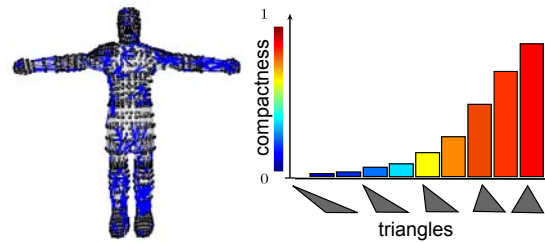
Figure 9: Dual-Graph Simplification (left) and Triangle Compactness (right).
