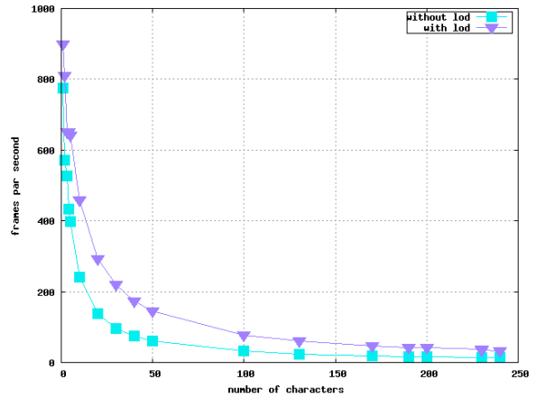
Figure 15: Benefit of skeletal Lod for crowds.
