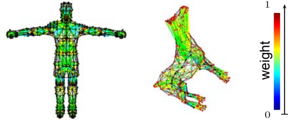
Figure 2: Binding.
