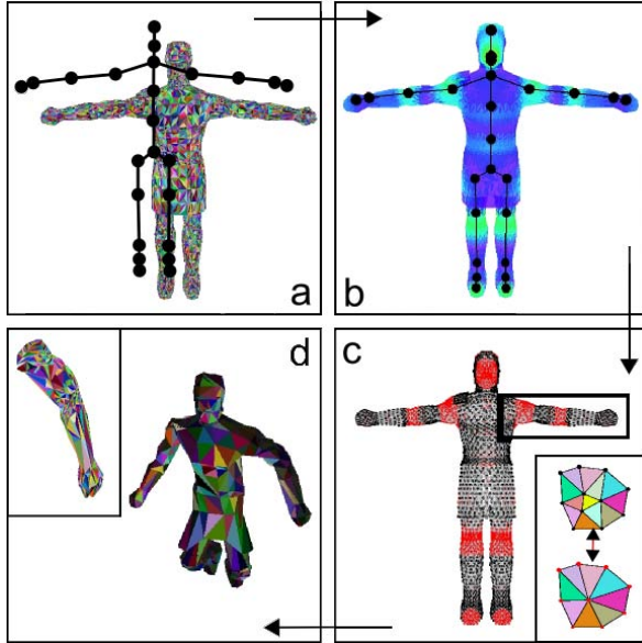
Figure 8: Multi-resolution mesh.
