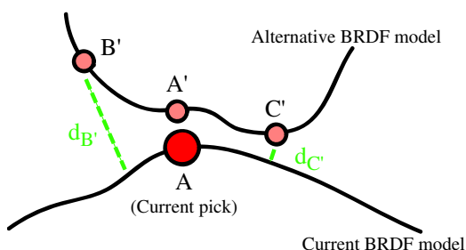
Figure 6: Illustration of the manifolds spanned by two analytical BRDF models in an abstract unified BRDF space. Point on the black curves represent instance of two BRDF models. Given a current BRDF, we want to find BRDFs on an alternative model that are close but cannot be represented by the current analytical model. We wish to propose materials such as B' because its distance d_{B'} to the current model is large. See text for detail.
