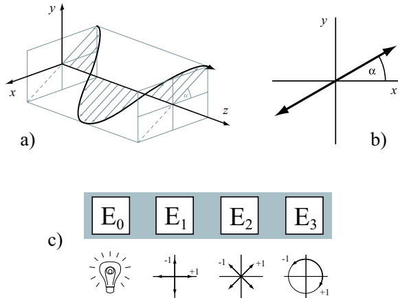
Figure 12: a) Three-dimensional view of the propagation of a linearly polarised lightwave which is rotated by an angle of \alpha from the x-axis. b) Two-dimensional view of the plane of oscillation for this wave. c) The Stokes Vector formalism: four numbers are used to describe the polarisation state of a wave. The first component E_0 encodes the total luminance, components E_1 and E_2 encode linear polarization in two different orientations rotated by 45^\circ , and E_3 is used to describe the circular polarisation component.
