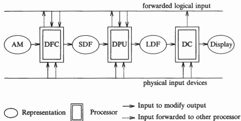
Fig. 1 Functional model of image generation pipeline (Carlbom 1 );
