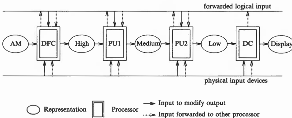
Fig. 5 Functional model of the proposed architecture;
