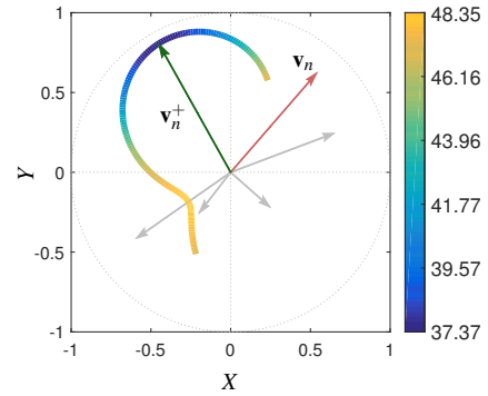
Figure 7: Optimal length visualization for updated vectors. When choosing a different orientation for an axis vector ( \mathbf{v}_n ) it is possible to use the solution to (20) to obtain an optimal length for it. The colored curve included in the plot shows the optimal lengths for axis vectors orientated between 68^\circ and 247^\circ . It also shows the direction the axis vector should point towards to (e.g., a vector orientated at 30^\circ \equiv 210^\circ should end up pointing towards the 3rd quadrant). The colors indicate the estimation error that would result by choosing a vector with its endpoint on the curve. Thus, \mathbf{v}_n^+ is the optimal vector for replacing \mathbf{v}_n .
