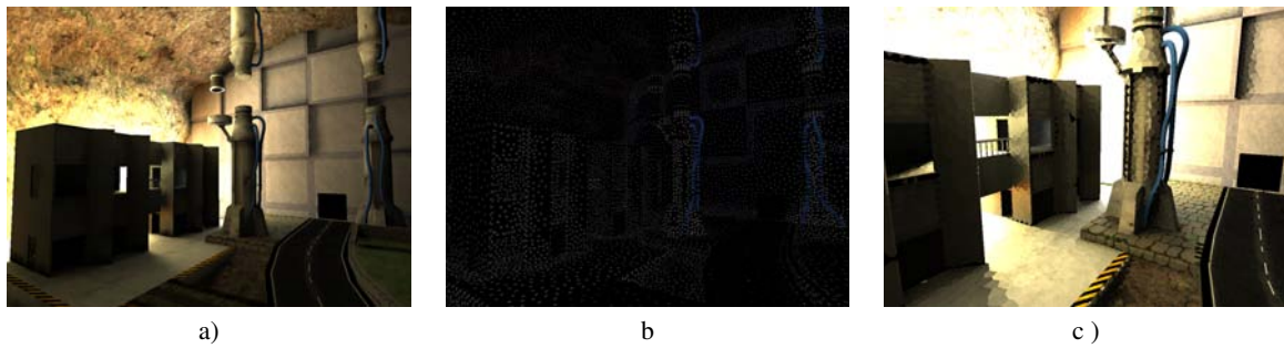
Figure 2: Rendering using the point set. a) Indirect lighting; b) Visualization of the point set; c) Voronoi diagram for the stored shading information. The size of the point set in these images is 120k, and was generated in less than 4 minutes.
