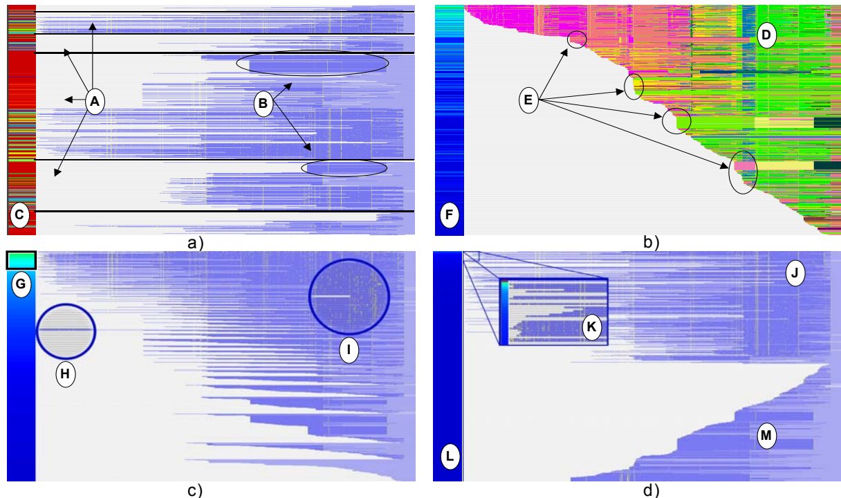
Figure 7: Interactively built layouts of the VTK project using sort operations: (a) files sorted alphabetically, vertical metric shows cluster IDs, (b) files sorted by creation time, vertical metric shows activity, (c) files sorted by activity, vertical metric shows activity, (d) files sorted by similarity with respect to a reference file- vtkIntArray.cxx , vertical metric shows similarity.
