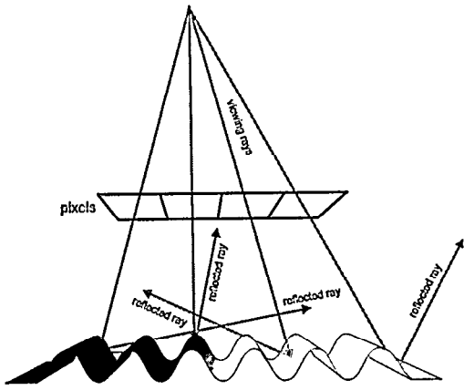
Fig. 3: Antialiasing of bump maps is necessary; otherwise we get rays reflected into random directions or random Phong illumination values.
