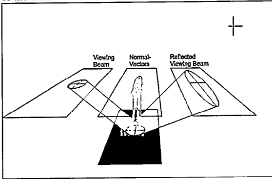
Fig. 8: The viewing rays contributing to a pixel form a beam. This beam is reflected by a bumpy surface into the reflected viewing beam. The shape of the reflected viewing beam is approximated using the distribution of normal vectors in the reflecting area by an elliptical cone. And yes: it could be argued that the normal vectors that end in the drawn ellipse, should be drawn starting from one origin, not from the surface location, they belong to. The same applies for the reflected beam.
