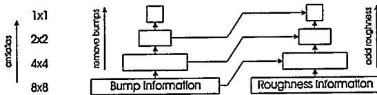
Fig. 9: Bump- and roughness pyramid
