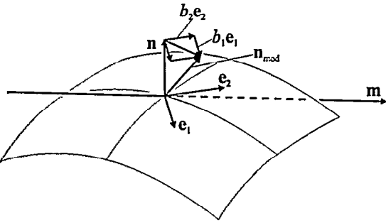
Fig. 7: The construction of the local coordinate system for the bump map using a main direction \mathbf{m} .
