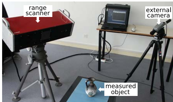
Figure 3: Our digitization bench to capture whole surface light fields. Only a lightweight device is involved: a structured light range scanner and an external camera.
