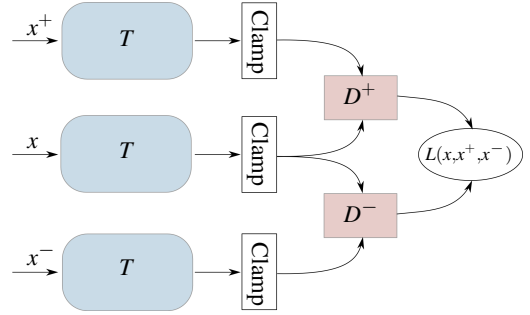
Figure 4: Our triplet network architecture consists of three convolutional neural networks T with shared parameters. Their outputs are then clamped such that \|T(x)\|_2 \leq 1 for any query, positive or negative sample, such that the embedding space is confined to a hyper-sphere. The embeddings of the similar and dissimilar sample are compared to the query in D^+ and D^- respectively. These relative distances are then compared in the triplet loss function (3).
