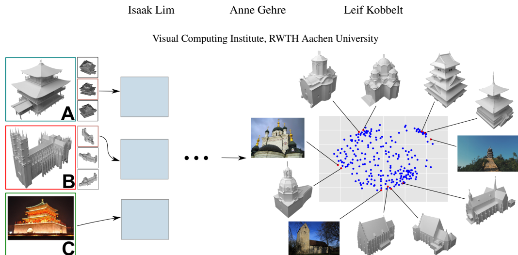
Figure 1: A high-level visualisation of our approach to style similarity learning using deep metric learning. To the left a triplet consisting of a query sample (A), a dissimilar (B) and a stylistically similar sample (C) is shown, i.e. B and C are compared to A. Triplets of this type are fed into a neural network consisting of three convolutional networks (blue boxes), which computes an embedding (right) of these samples. The embedding space (here illustrated by multi-dimensional scaling) is such that stylistically similar samples are placed close together while dissimilar samples are placed further apart. By using rendered images as a representation for 3D shapes we are able to incorporate photos found online [pix]. This reduces the cost and effort to compile the training set since annotated images are broadly available while annotated (and consistent) 3D models are more difficult to get.
