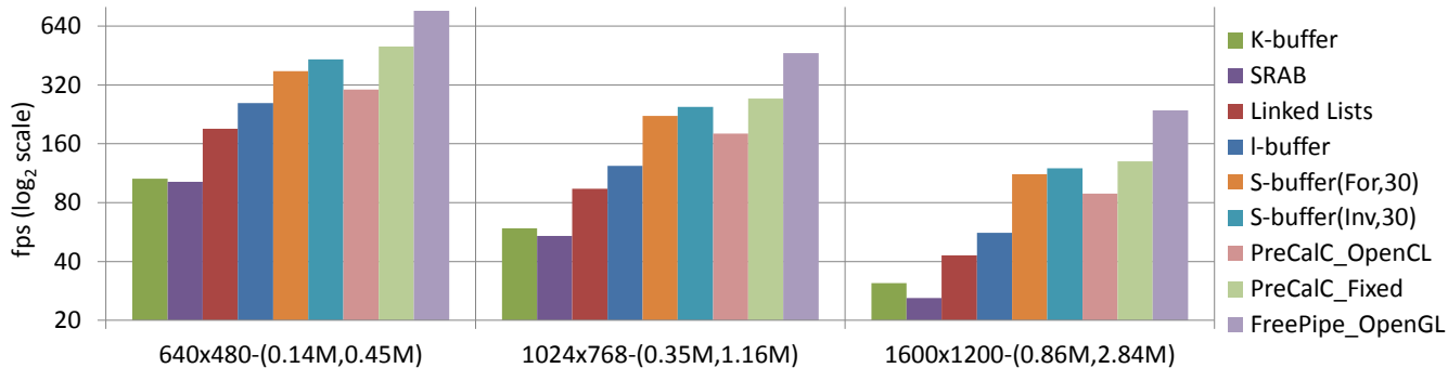
Screen resolution-(used pixels, generated fragments)
