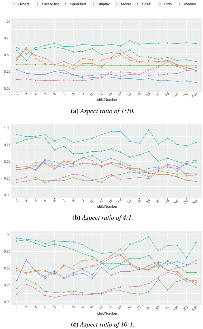
Figure 2: Measurements for 3 out of 13 different aspect ratios (2a, 2b, 2c) of the generated datasets showing the layout quality score (y-axis) in relation to childNumber (x-axis).
