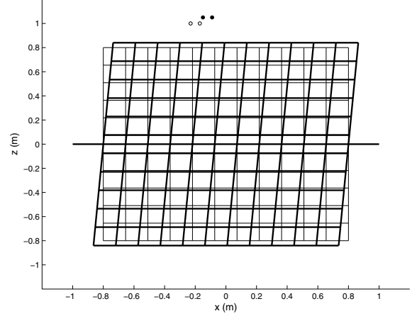
Figure 5: The effect of head position error. The perceived virtual space appears expanded and sheared. The modeled and true eye locations are represented by the empty and filled circles, respectively. The thin grid indicates the true workspace, the thick one is the perceived counterpart.
