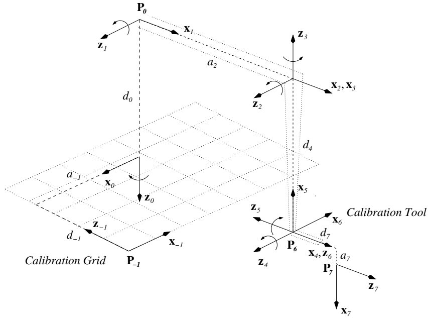
Figure 3: Kinematic model of the PHANToM 3.0L mounted in the overhead configuration (T model). The stylus is augmented with a calibration tool for taking measurements on the display surface of the workbench.
