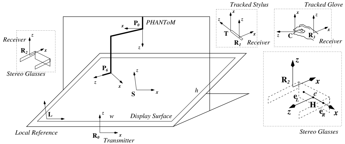
Figure 2: Coordinate frames effecting display accuracy of the Visual Haptic Workbench. Possible sources of error include individual device workspace distortions and misalignments of the respective coordinate systems.
