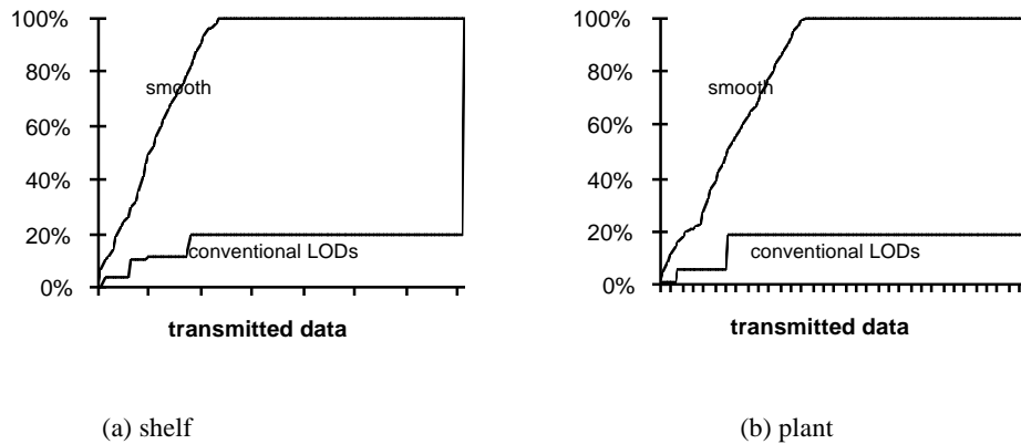
Figure 35: Comparison of visual effect of smooth vs. conventional LODs. We measured the quality as the number of triangles available for a certain amount of data (1 notch on the x-axis \approx 5 KB)
