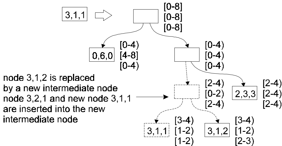
Figure 23: Inserting a vertex into an occupied subvolume
