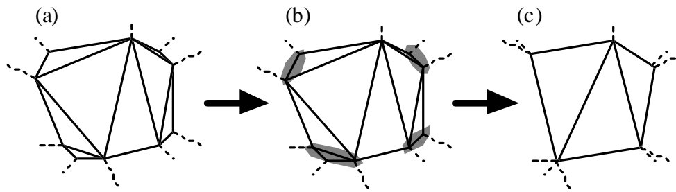
Figure 32: The clustering process: A mesh (a) is mapped onto a vertex cluster tree, which is used to group vertices (b). From the reduced vertex set, a simplified model (c) is computed.
