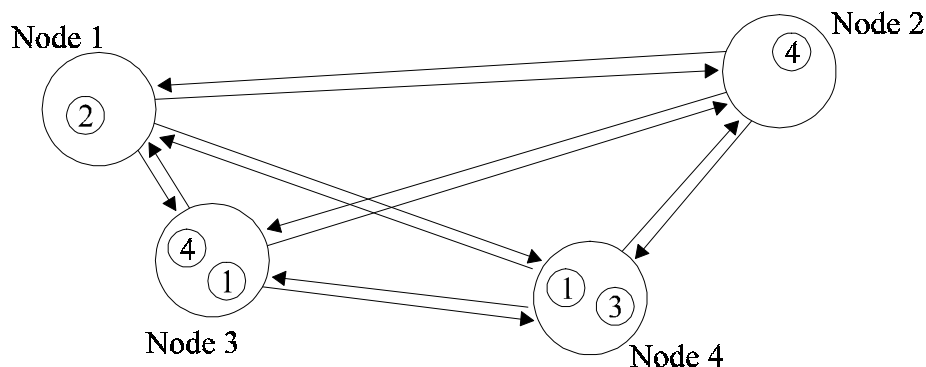
Figure 6: Peer-to-peer unicast network topology. In this example, large circles represent network nodes, each one occupied by one user. The small circles with numbers represent the avatars of other users (nodes) that must be simulated and displayed locally. Arrows indicate the flow of update information according to the individual needs for local simulation.
