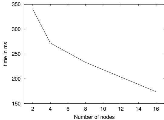
Figure 7: Scalability of the visualization system with the number of rendering nodes.
