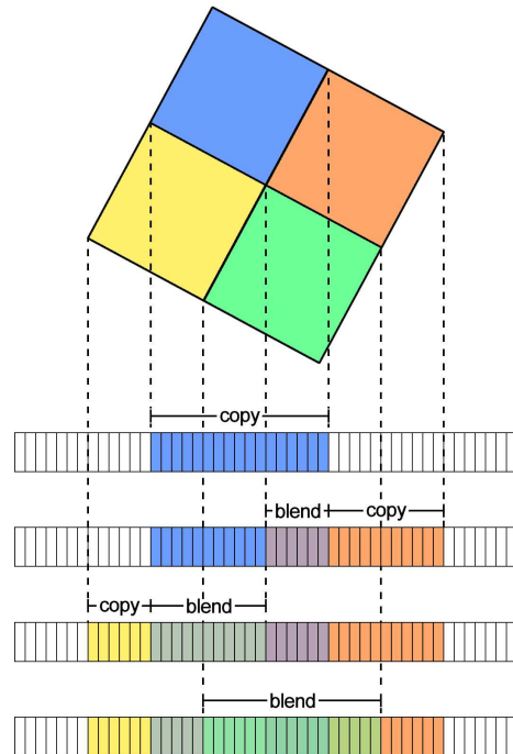
Figure 1: Depth-sorted blending of footprints of four volume blocks. For each compositing step the regions with and without the need for blending are marked.
