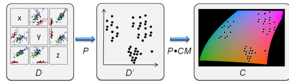
Figure 3: Schematic Approach. High-dimensional data D is projected with P to low-dimensional space D' , which is transformed with P \bullet CM to fit into color space C .
