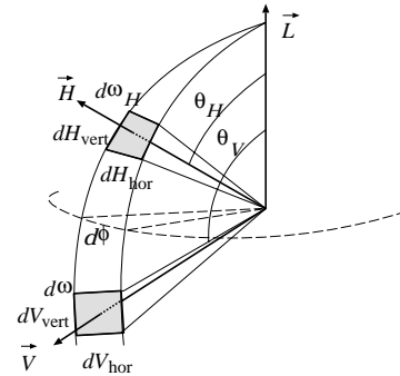
Figure 9: Calculation of d\omega_{\vec{H}}/d\omega_{\vec{V}}
