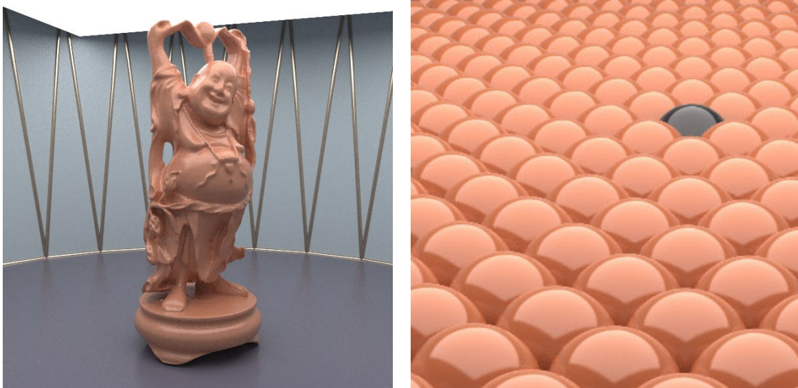
Figure 7: Scenes of plastic Buddha and balls. The index of refraction used by the Fresnel function is 1.7 and the roughness parameter m is 0.03. The Buddha model is from the Stanford 3D Scanning Repository ( http://graphics.stanford.edu/data/3Dscanrep/ )
