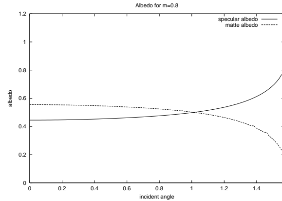
Figure 5: Albedo curves of the specular and matte components for m = 0.8 . The total albedo is 1.
