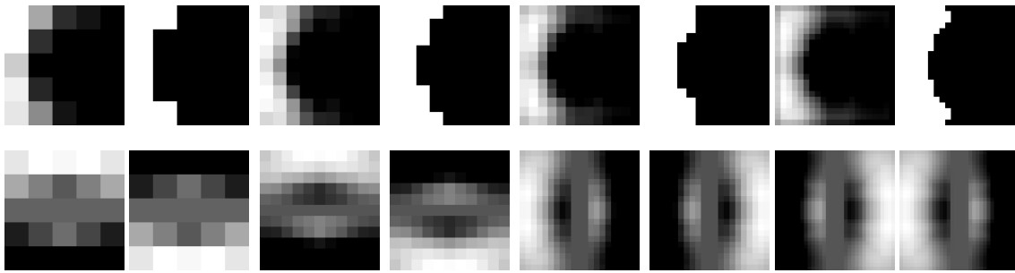
Figure 1: Optimised masks derived with our criterion: the first row shows depth from defocus masks with resolution n = 5, 9, 13, 21 together with their thresholded versions. The second row shows coded-aperture pairs of resolution n = 5, 11, 21, 33 .
