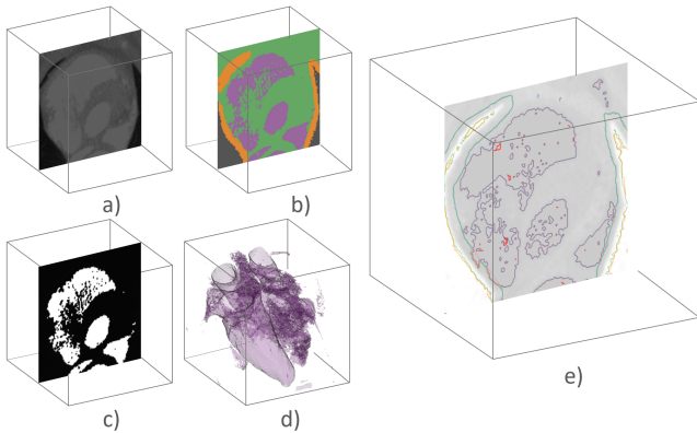
Figure 3: Computational workflow for the presented approach. a) Original slice of the input volume. b) Resulting Clustering of the error space using k-means clustering ( k = 4 ). c) Resulting weights for the first cluster. d) Iso-surface visualization of the first cluster using 0.5 as iso-value. e) Embedding of iso-lines from all cluster into the slice-by-slice reviewing method.
