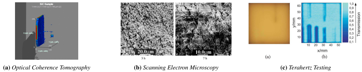
Figure 4: (a) Optical Coherence Tomography: OCT image of a silicon carbide. For the 3D representation, multiple OCT scans have been performed, each 10\ \mu\text{m} deeper than the one before. Color encodes the strength of the backscattered signal from red (strong) to blue (weak signal). At z -values close to 0 the scattering is extreme due to the transition from air to material. Inside the material two scatterings are observed representing defects: The thin line normal to the surface and the big spot in the bottom right corner. ©1998 Optical Society of America. Reprinted, with permission, from [DBR98]. (b) Scanning Electron Microscopy: SEM image of a surface membrane exposed to a fouling process after 3 and after 7 hours. After 7 hours the complete membrane is covered with calcium carbonate. Even with higher resolution no empty spots are found. Reprinted from [SLKL02], with permission from Elsevier. (c) Terahertz Testing: THz imaging of a plastic specimen with drilled holes. (a) shows a photograph of the sample. (b) shows the corresponding THz image. The drilled wholes are clearly visible using THz imaging. ©2010 Optical Society of America. Reprinted, with permission, from [JWP*10].
