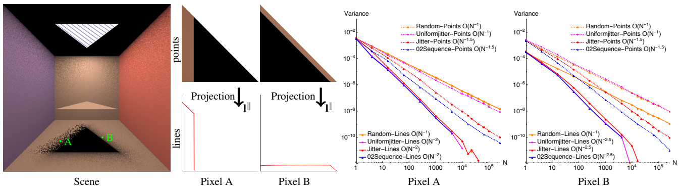
Figure 5: Line orientation: We analyze the impact of line sample orientation on variance and convergence rate. Line samples on the light source are generated parallel to the edge above pixel A. Consequently, the regions below the left side of the triangle occluder see a step function (shown for Pixel A in second column) and benefit only from dimensionality reduction. The other two sides of the occluder benefit from both dimensionality reduction and smoothing of the integrand (shown for Pixel B in the second column).
