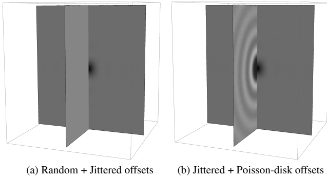
Figure 2: Bidirectional line sampling leads to expected power spectra constrained to the two planes of sample offsets (shown axis-aligned here for clarity). The line offset sampling process for each direction determines the spectrum within the corresponding plane (shown here for combinations of random, jittered, and Poisson-disk).
