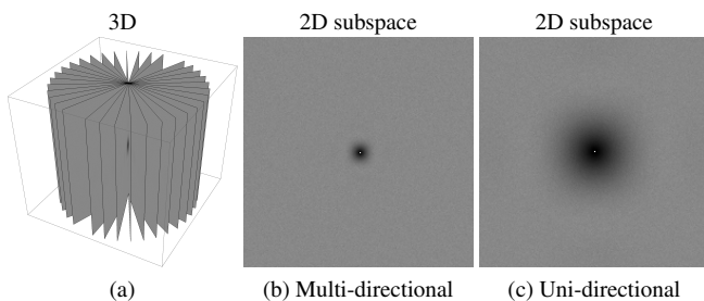
Figure 3: We analyze the multi-directional expected power spectrum (a) with m = 16 directions and N_k = 256 jittered line samples along each direction k , for a total of N = 4096 line samples in 3D. The dark region around DC for each 2D subspace (b) shrinks with more directions compared to the unidirectional case (c).
