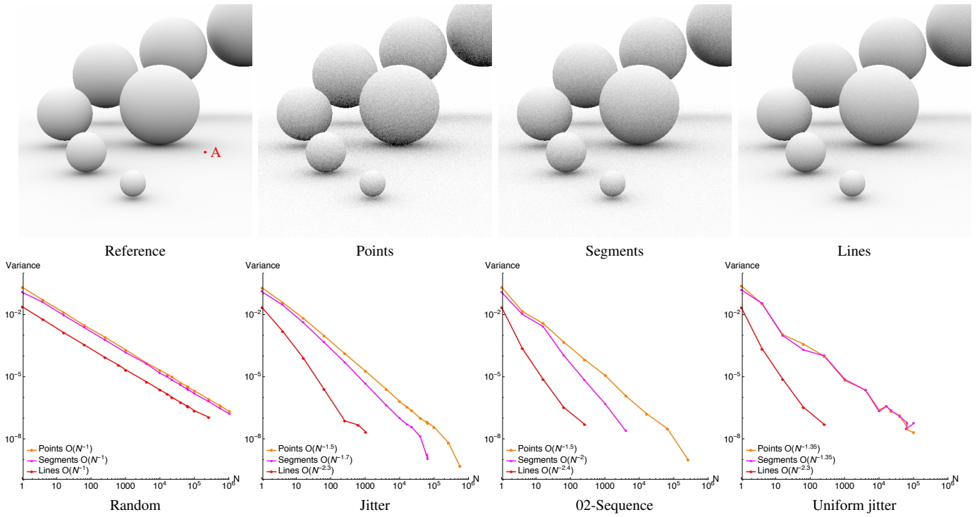
Figure 6: Points, Segments & Lines: In the top row, we show the ambient occlusion scene which is rendered with N = 16 jittered points, segments (of length = 1 radian) and line samples. The reference image is generated with N = 1024 jittered line samples. The bottom row compares the improvements using segment and line samples over point samples for four different samplers at Pixel A (marked in red in the reference image). For more comparisons please refer to the supplemental Fig. 1.
