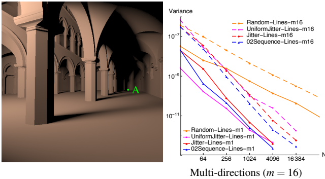
Figure 7: Multi-directions: We generate 16 point samples per pixel and perform line sampling in a direction associated to each pixel sample with a fixed sample count.
