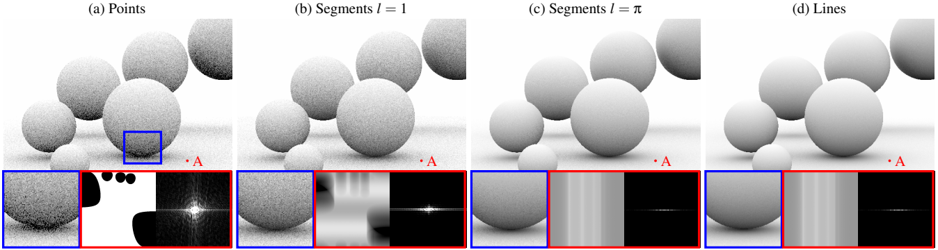
Figure 8: Points, Segments & Lines: We compare the impact of segment length ( l ) on the variance for the ambient occlusion scene. All renderings are performed with N = 9 jittered samples. Inset in blue is the zoom-in region of the sphere at the center (marked in (a)). The insets in red visualize the integrand for Pixel A and the corresponding power spectrum. As the segment length increases, variation of the pre-filtered integrand (and its power spectrum) diminishes along the vertical axis due to the convolution by the segments. For length l = \pi , segments cover the full \theta range like line samples, however, the variance due to these long segments is still higher compared to line samples. This is because, by construction, segment centers span a 2D domain while line offsets span a 1D domain, and can leverage denser 1D stratification. For more comparisons please refer to the supplemental Figs. 2, 3 & 4.
