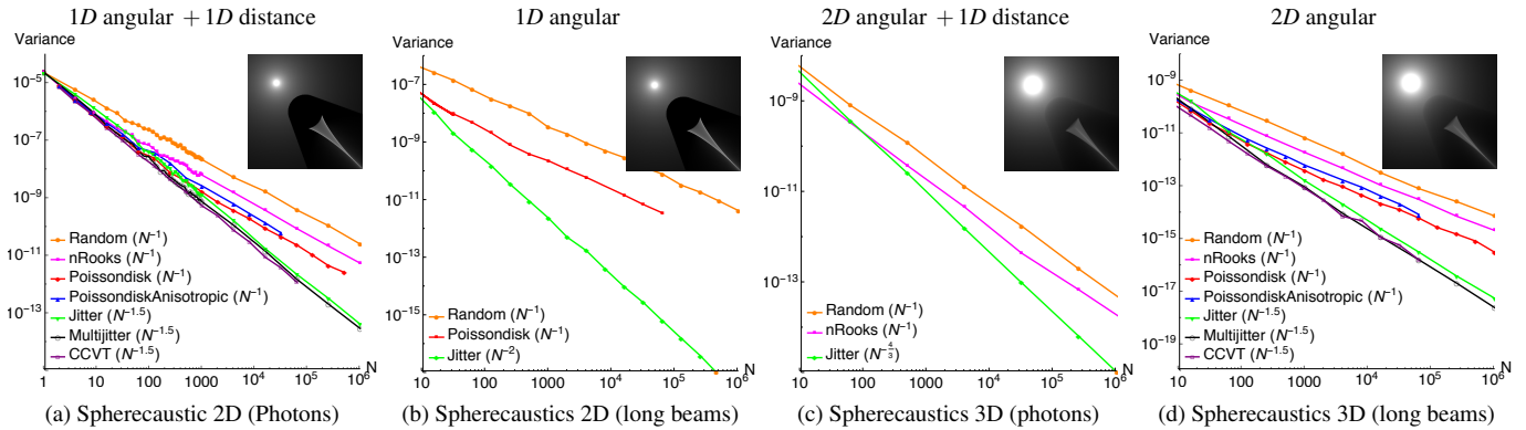
Figure 9: Points & Lines: We analyze the variance convergence rates for a homogeneous participating medium which is rendered in 2D (flatland) and 3D using photons (a, c) and long beams (which are photon beams that analytically compute transmittance along each direction) in (b, d). On the top, we are showing the sampled dimensions for each case.
