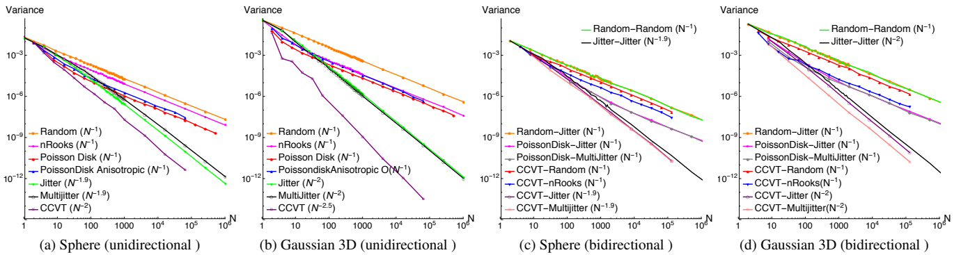
Figure 4: Line samples 3D: Empirical variance convergence rates for the worst (Sphere) and the smooth (Gaussian 3D) case functions integrated using various unidirectional (a,b) and bidirectional (c,d) line sampling patterns. With jitter and CCVT, Gaussian (b) follows the convergence rate for d = 2 from Table 1 for this 3D integral. However, for the sphere (a), the experimental convergence rate is much better than the theoretical one shown in Table 1 for d = 2 . This is because line samples not only reduce the dimensionality but also prefilter the C_0 discontinuities in the case of sphere. In (c,d), the convergence rate is dominated by the direction with samples having worst convergence.
