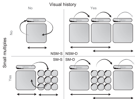
Figure 5: Four different tested interaction methods involving combinations of Small Multiples and Visual History.
