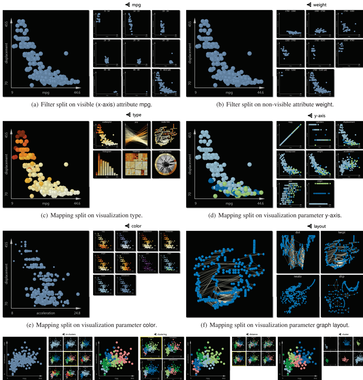
Figure 3: Generation of Small Multiples by splitting Large Single.
