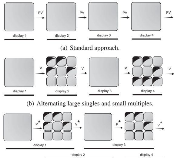
(c) Showing a large single and small multiples alternating in one display allowing for multiple operations.
