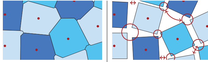
Figure 7: Voronoi cells (left) and materialized cubes (right). Due to the cell's keystone, the distances between virtual vertices may vary significantly and is therefore not a robust criterion for a merge.
