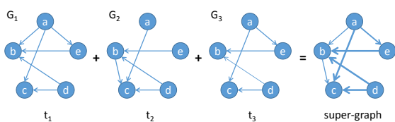
Figure 6: Constructing a super-graph from a dynamic graph with three time-steps; edges occurring in multiple time steps are aggregated by higher edge weights (line thickness).
