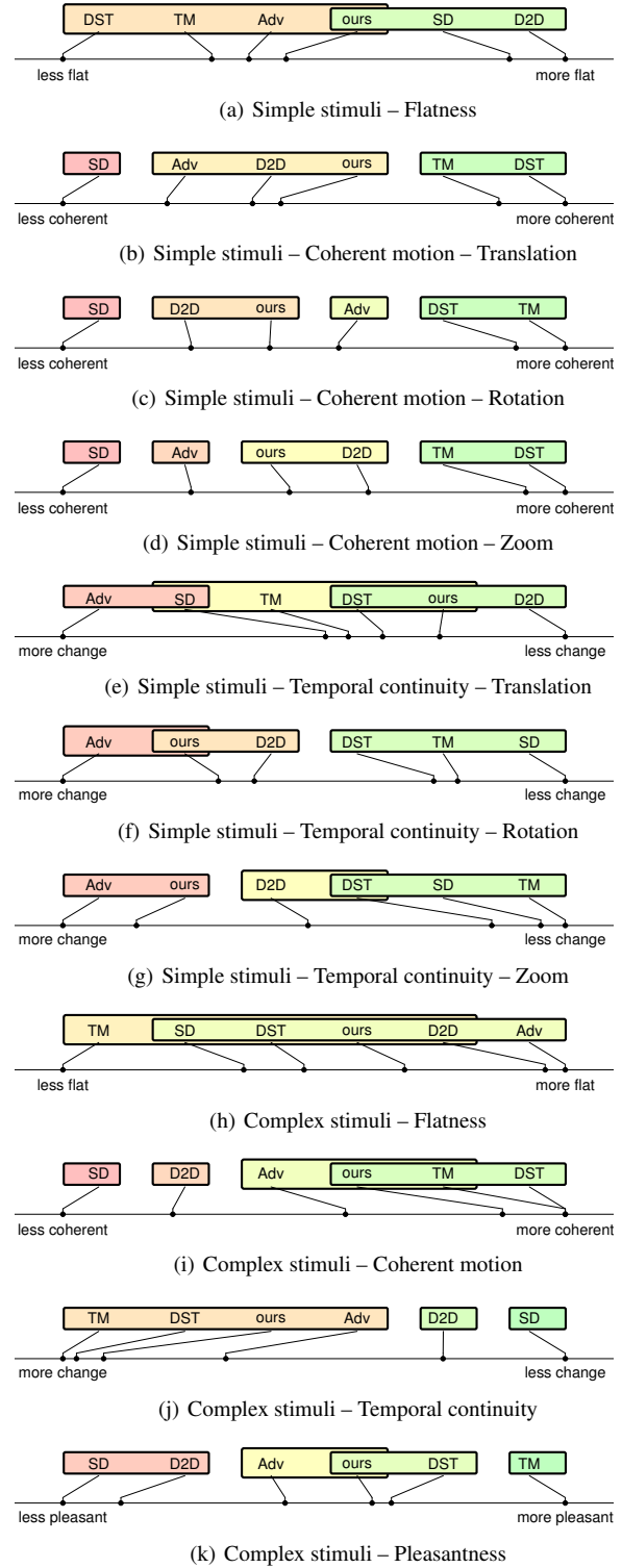
Figure 2: Interval scales indicating the relative merits of each method. The methods are classified into similarity groups based on the Wilcoxon rank-sum hypothesis test at 95% significance level.
