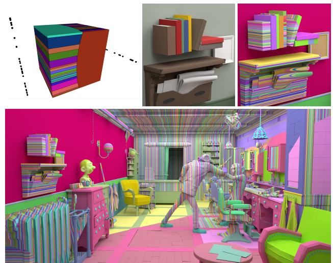
Figure 1: Pathological configuration for state of the art methods. Sites are distributed on axis aligned lines far from the domain (top left) which makes the full diagram complex. On a 6D (x,y,z,r,g,b) scene with 2M faces and using 100k sites on 20 lines (bottom) we compute the restricted diagram in 43s while other methods cannot compute it in a reasonable time. Note how regions with different input colors (middle top) are clipped by different sites (top right). Agent 327 scene courtesy of Francesco Siddi, Blender Cloud.
