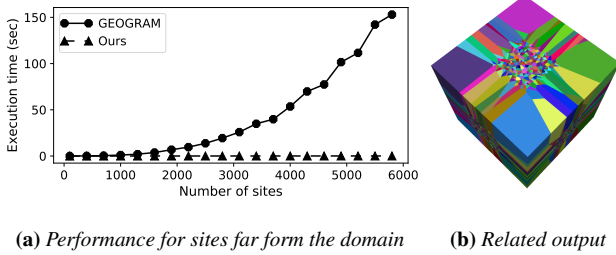
Figure 12: (a) Performances of our algorithm compared to GEOGRAM configured with security radius [LB12, Lév16]. Their performance for sites far from the domain drops while our algorithm scales smoothly (see § 2.3.2.3 and Section 5.3).
