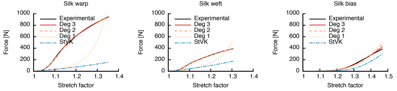
Figure 3: Demonstration of the improvement of fit quality as the model complexity increases for silk. For warp and weft, degree 2 is sufficient to fit the experimental data well (average relative error under 2%). For bias, the transition from degree 2 to 3 still makes significant progress (average relative error reduces from 6% to 4.5%). In all cases, an orthotropic St. Venant-Kirchhoff model provides a poor fit. Due to our minimization of relative error, the small strain regime is prioritized even when using models too simple to match the full curve. For the remaining fabrics, the final curve degrees for warp, weft, and bias respectively were 3, 3, and 2 (cotton); 2, 3 and 3 (canvas); 5, 5, and 4 (denim); and 5, 5, and 3 (wool).
