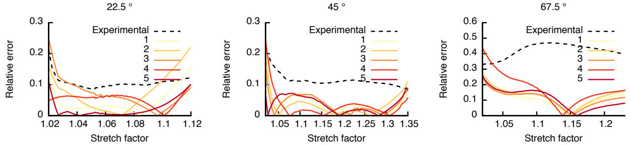
Figure 4: Relative error plots for tensile tests at 22.5°, 45°, and 67.5° after adjusting for accidental cloth sample misalignments. The black curve shows the relative difference between the largest and the smallest unadjusted force measurements. Each of the remaining curves show the relative error of the model fit compared to the experimental data for one cloth specimen. With very few exceptions the fitting error is well below the experimental error.
