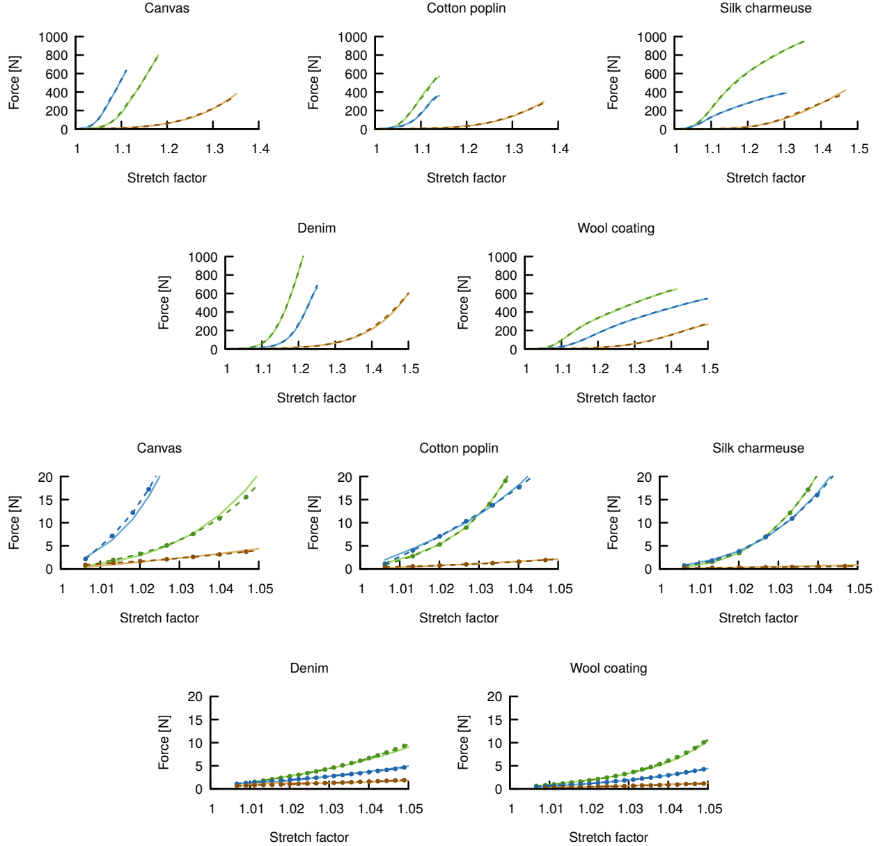
Figure 2: Force-elongation curves for 5 cm wide strips of canvas, cotton, silk, denim, and wool. Measured data is shown with dashed lines while fitted curves are shown in solid. The top set of plots shows the full strain domain while the bottom set shows a closeup for the small-strain regime. Each plot shows curves for warp (green), weft (blue) and bias (brown). Dots represent data points but are only shown in the small strain plots for legibility.
