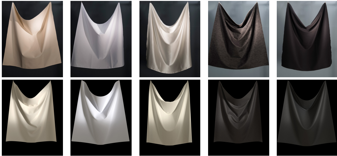
Figure 1: Photographs of five fabrics (canvas, cotton poplin, silk charmeuse, denim and wool coating) along with the corresponding simulation after parameter estimation (bottom row). Each piece of fabric is 1\text{m} \times 1\text{m} , and the top corners are held 60cm apart. The real fabrics had multiple stable equilibria for the specified constraints, so exact matches cannot be expected.
