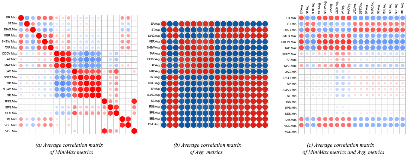
Figure 6: (a) shows the correlation matrix of Min/Max metrics, (b) shows the correlation matrix of Avg. metrics, while (c) shows the correlation matrix among Min/Max metrics and their corresponding Avg. metrics. Note that the metrics in the matrices shown in (a–b) are re-ordered based on the clustering result shown in Figure 5. The sizes of the dots indicate the strength of the correlation, while red means positive correlation and blue means negative correlation.
