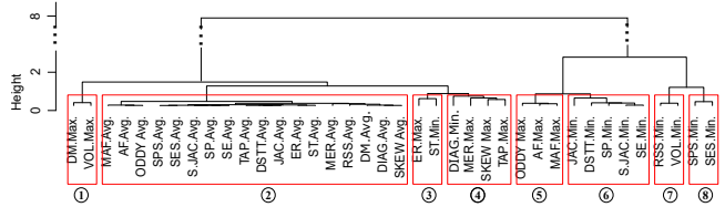
Figure 5: Hierarchical clustering result of all the quality metrics listed in Table 1 and their corresponding average metrics.
