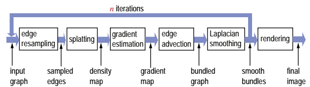
Figure 3: KDE edge bundling pipeline.
