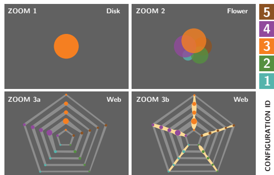
Figure 3: The proposed glyph set enables details-on-demand using zoom levels. The levels have a coherent transition and provide progressively rich information. The first level shows a disk glyph that conveys the overall maximum WSS. By zooming in, the flower glyphs shows the maximum WSS over time for each stent configuration. The web glyph furthermore conveys the WSS variations in time, first as a subsampling (3a) and finally with time variation strips (3b).
