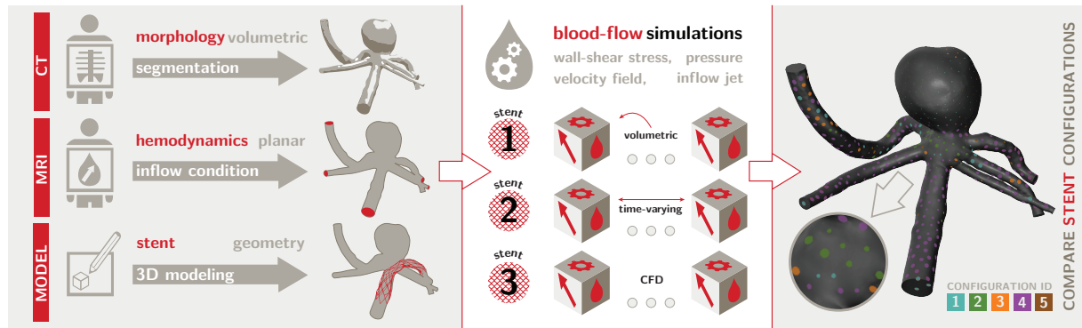
Figure 1: An overview of the data analysis pipeline. On the left-hand side, the simulation inputs are depicted. Patient-specific morphology is obtained by segmentation of computed tomography (CT) imaging data. Together with this geometry, inflow conditions and different stent configurations are used to model the blood flow behavior. The blood flow simulations, shown in the middle, provide for each stent configuration a time-varying volumetric velocity field, as well as vessel wall characteristics. Visual analysis of this abundance of information is tedious and time-consuming. Therefore, we present a comprehensive comparative visualization that supports the decision-making process for stent placement, as depicted on the right-hand side.
