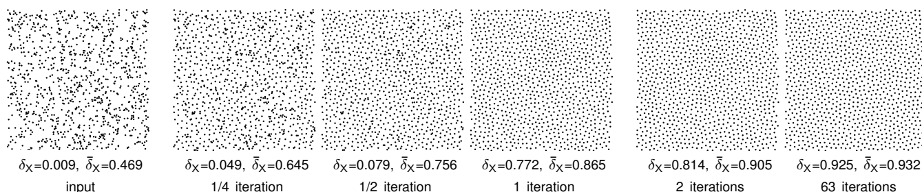
Figure 1: Farthest-point optimization of a random point set with 1024 points. Both the global minimum distance \delta_X and the average minimum distance \bar{\delta}_X increase rapidly using our optimization technique. After one iteration the point set is already well-distributed.
